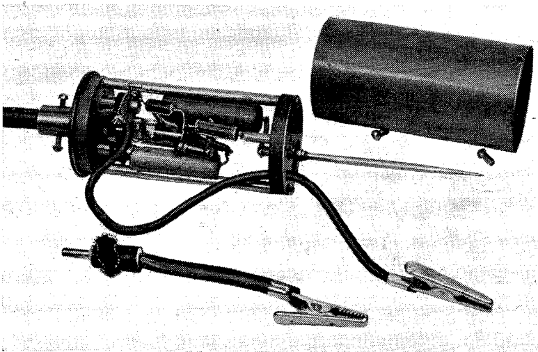
Valve voltmeter head with cover removed.
