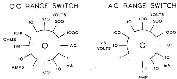
Fig. 1. Arrangement of twelve-position range switches.
