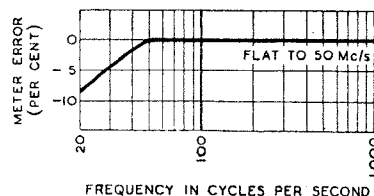
Fig. 5. Frequency characteristic of valve voltmeter.
