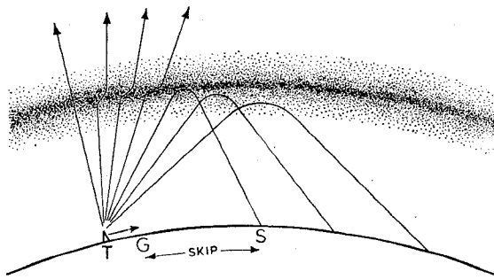
Fig. 6. The phenomenon of skip distance. T-G, range of ground wave; G-S, skip zone.
