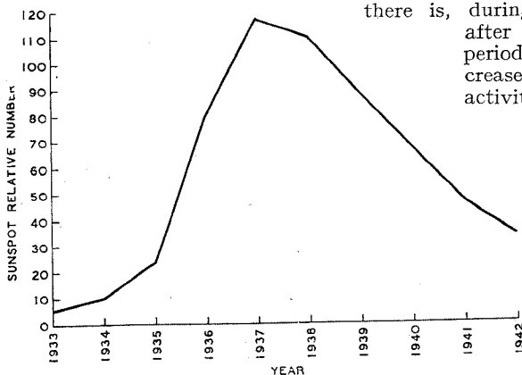
Fig. 1. Annual means of sunspot numbers during the present solar cycle.
